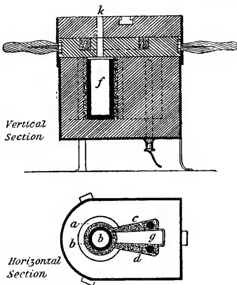
FIG. 44.—Furnace for granular heating material.
